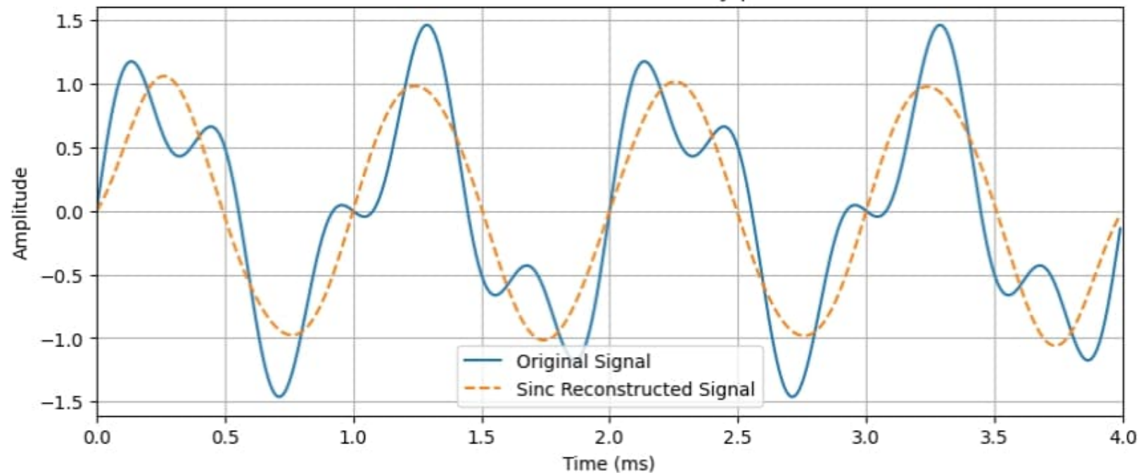
Sinc Reconstruction - At Nyquist
