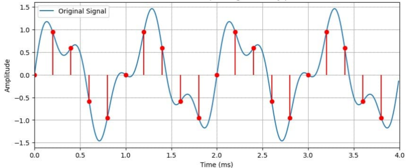
Reference and Sampled Signal - At Nyquist
